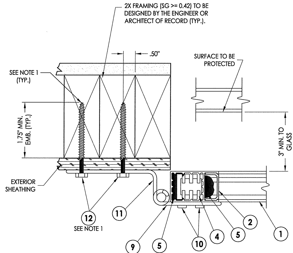
3 4 HORIZONTAL CROSS SECTION Stud construction
