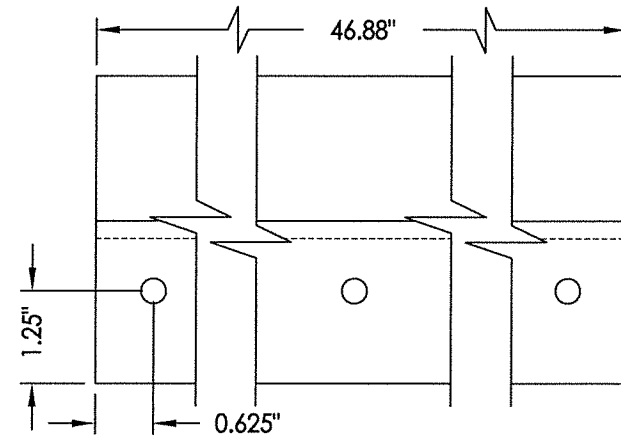
19 "Z" CLIP EXTENDED LATCH ALUMINUM 6063-T6
